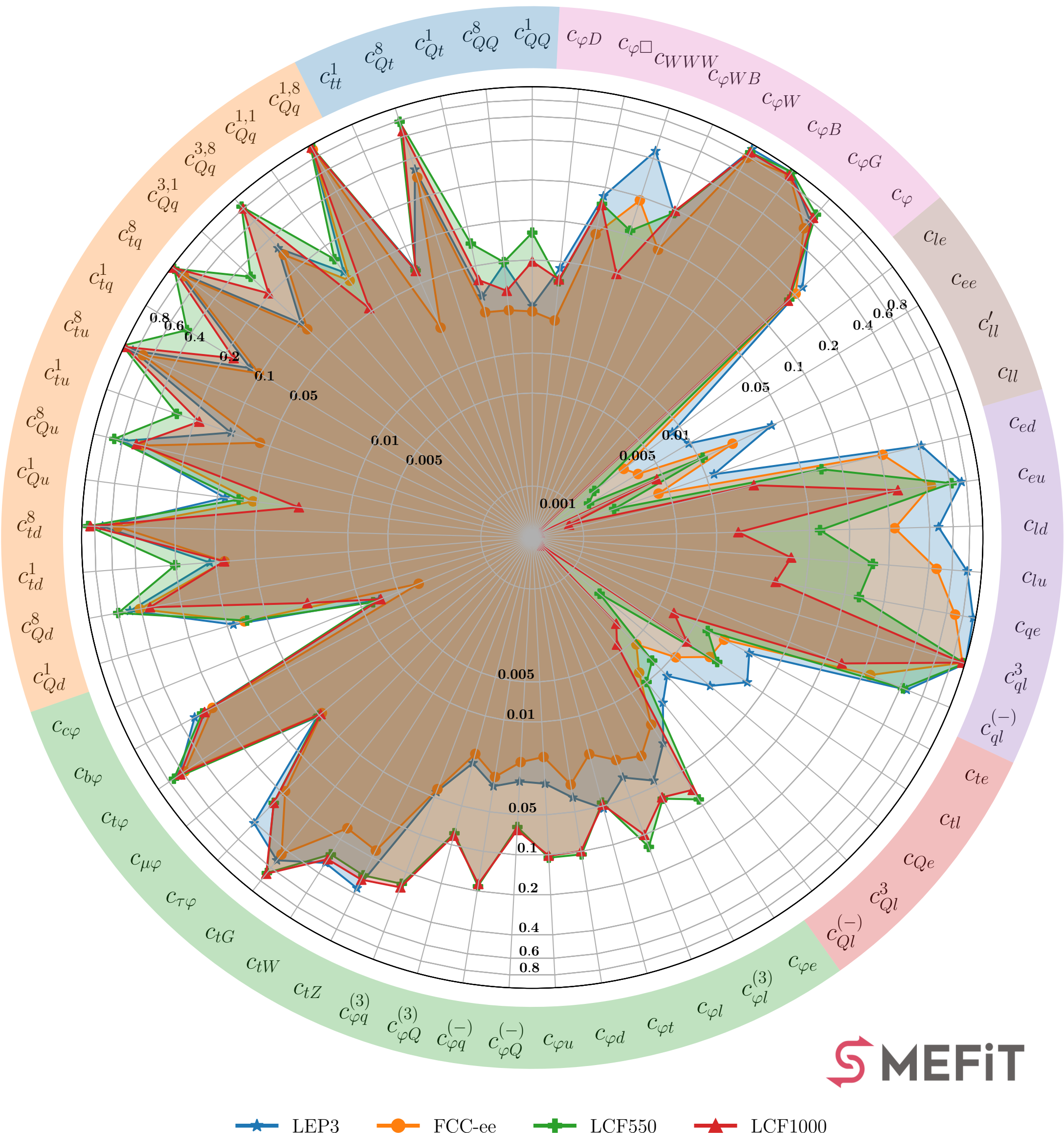
Ratio of Uncertainties to HL-LHC Baseline \mathcal{O}(\Lambda^{-4}) , Individual
